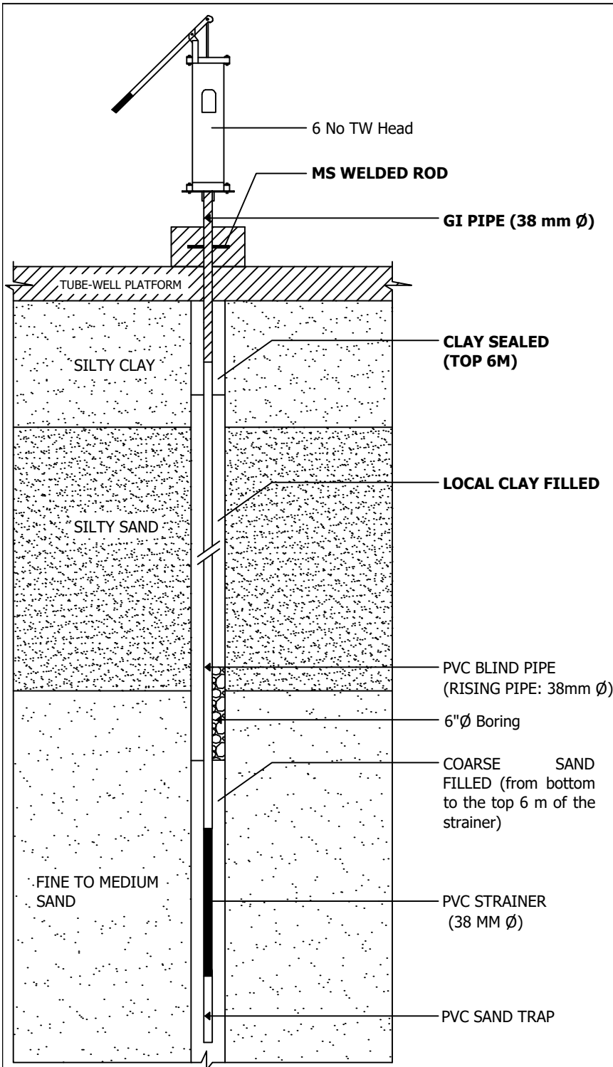
DIFFERENT COMPONENT OF TUBE-WELL
